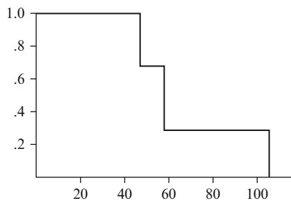
Figure 8.3. S_{2m}(t) : Survival to 2nd Event (Marginal)
