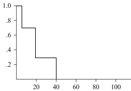
Figure 8.2. S_{2c}(t) : Survival to 2nd Event (Stratified GT)
