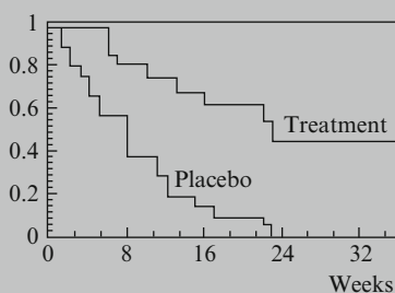
Expected Survival Plots by Rx Group Using PH Model
