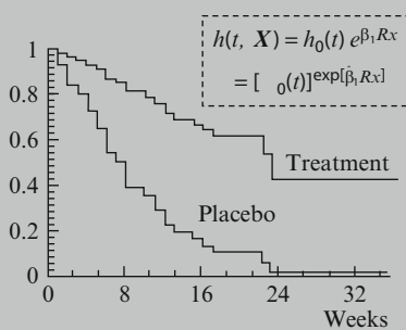
Expected Survival Plots by Rx Group Using PH Model
